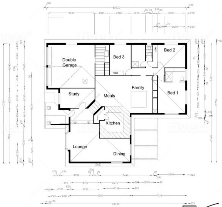
Floor Plan
