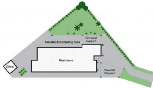
Site Plan
